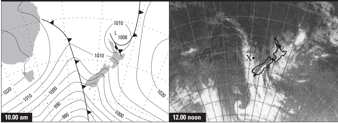
Source G — Synoptic Chart and Satellite Image for 2 December 2000
